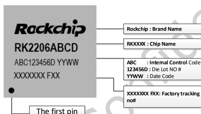
Fig.2-1 Package definition
