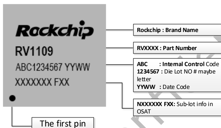
Fig.2-1 Package definition
